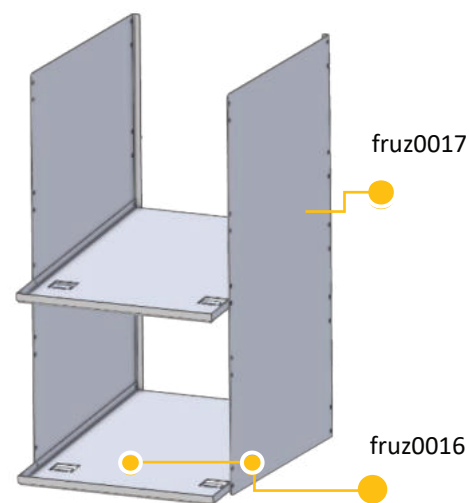
setLfruz015 (consists of 2x fruz0017, 2x fruz0016)
